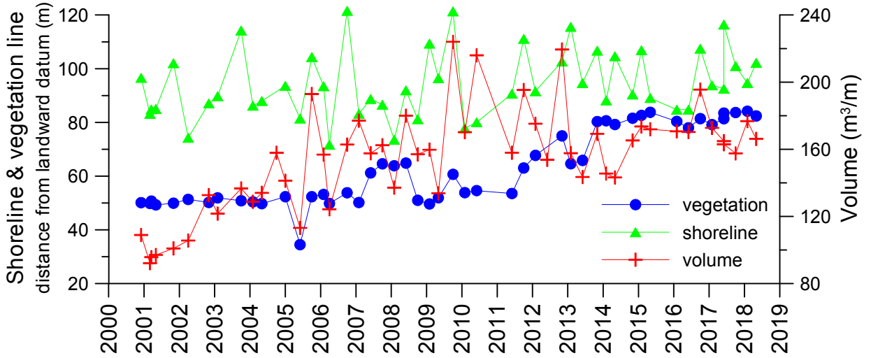
MUI02 (Mustang Island State Park) Volume, Shoreline, and Vegetation Line Change
