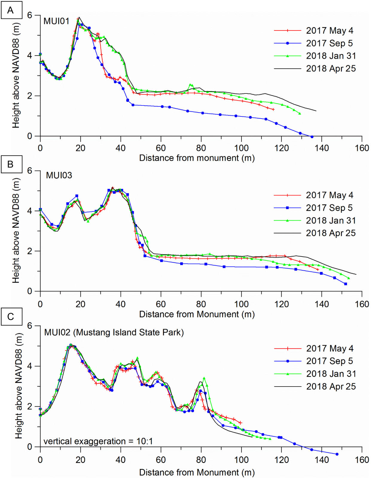
Figure 25. Mustang Island pre- and post-Hurricane Harvey profile data collected by Port Aransas High School and Texas A&M University Corpus Christi at (A) MUI01, (B) MUI03, and (C) MUI02.
