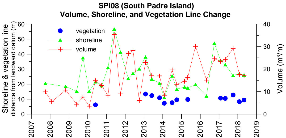
Figure 27. Sand volume and shoreline position changes at SPI08 on South Padre Island due to beach-nourishment projects and the installation of sand fences.
