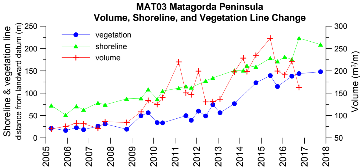
Figure 21. Changes in beach and dune volume, shoreline position, and vegetation line position at MAT03 on Matagorda Peninsula.
