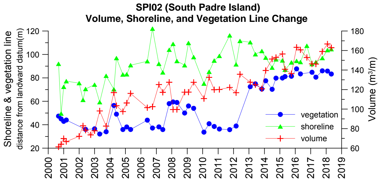
Figure 26. Changes in sand volume and shoreline and vegetation line position at SPI02 on South Padre Island due to beach-nourishment projects and the installation of sand fences.
