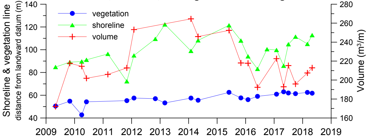
NPI08 (North Padre Island) Volume, Shoreline, and Vegetation Line Change
