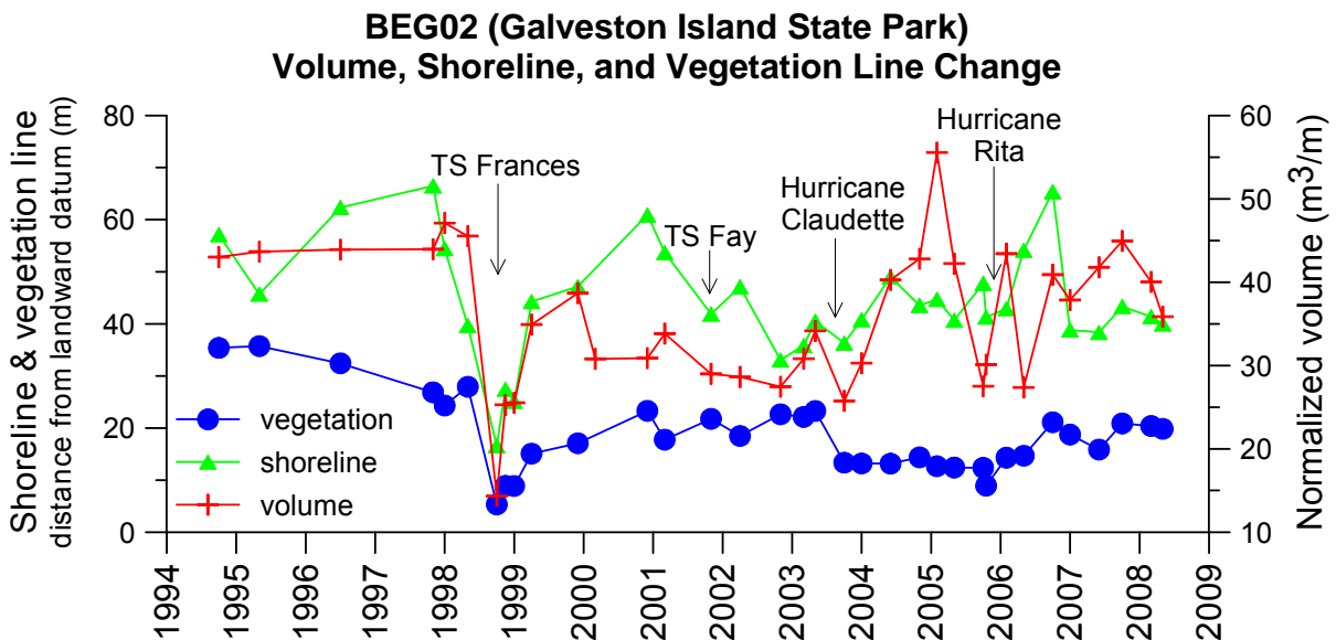
Figure 15. Profile volume, shoreline, and vegetation-line changes at Galveston Island State Park, September 1994–April 2008.
