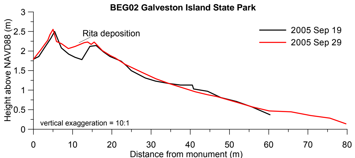
Figure 16. Plot of pre- and post-Hurricane Rita beach profiles measured at Galveston Island State Park.
