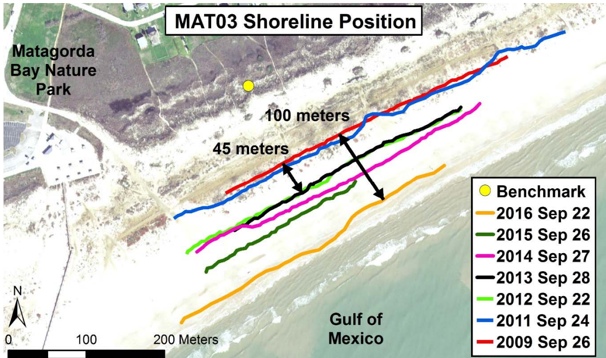
Figure 20. Shoreline position change at Matagorda Peninsula.
