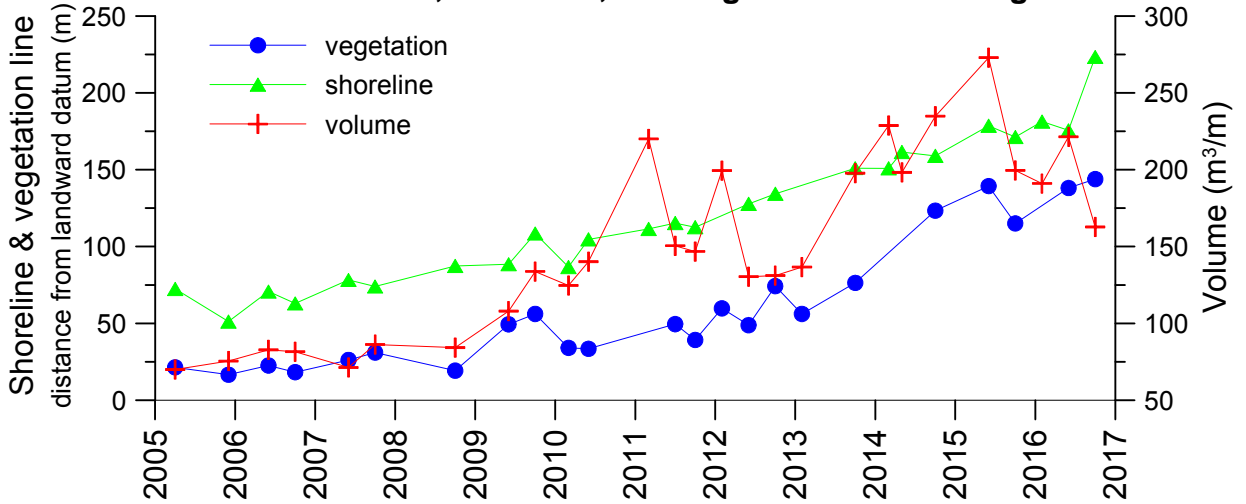
MAT03 Matagorda Peninsula Volume, Shoreline, and Vegetation Line Change
